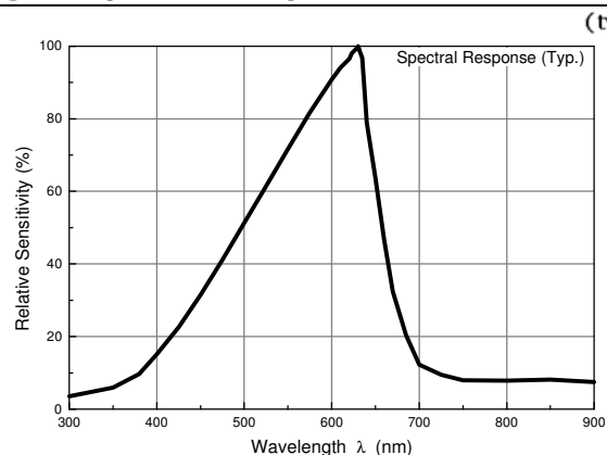
Fig.3 Spectral Response
